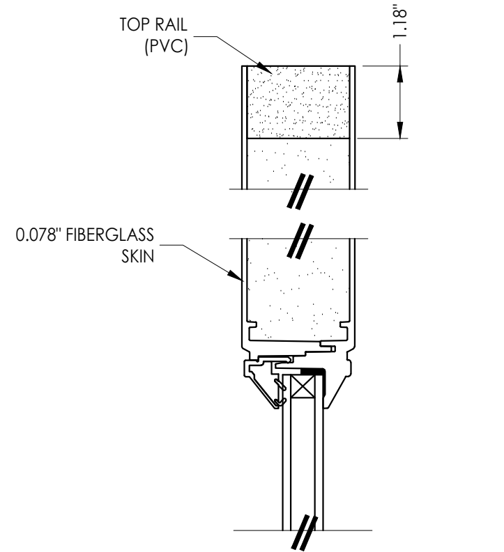
2 3 VERTICAL CROSS SECTION
