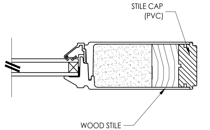
1 3 HORIZONTAL CROSS SECTION
